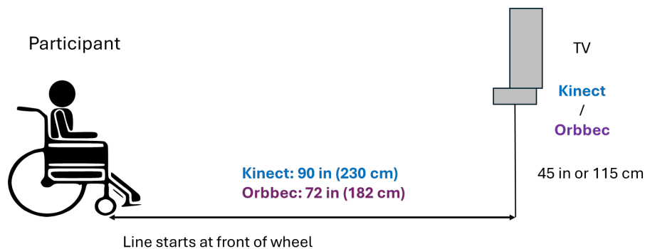
Figure 3: Kinect setup for patient in wheelchair. Side View.
